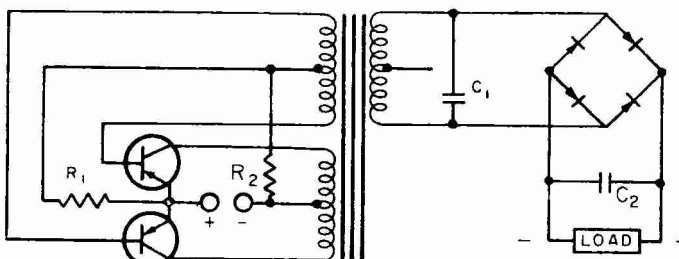
TYPICAL CIRCUIT
