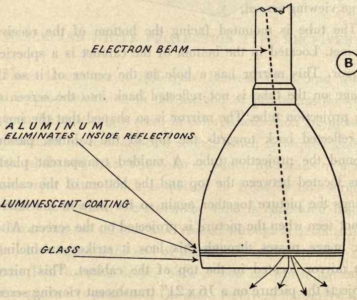
(A) OLD TYPE RECEIVING TUBE (B) NEW TYPE RECEIVING TUBE
