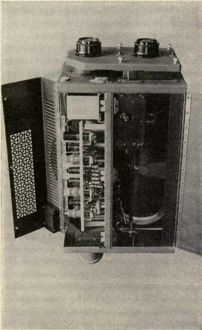
INSIDE VIEW OF STANDARD PICKUP CAMERA
