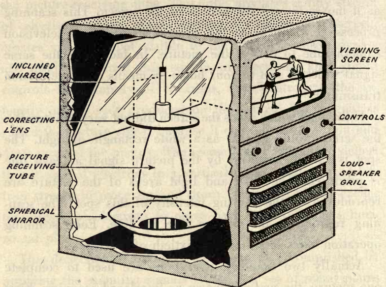
BLACK AND WHITE PROJECTION TYPE RECEIVER
