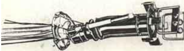
the Du Mont Bent-Gun used in all current Teletrons
