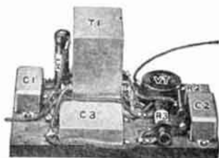
Television Chassis with Synchronizing Amplifier and Framing Device
