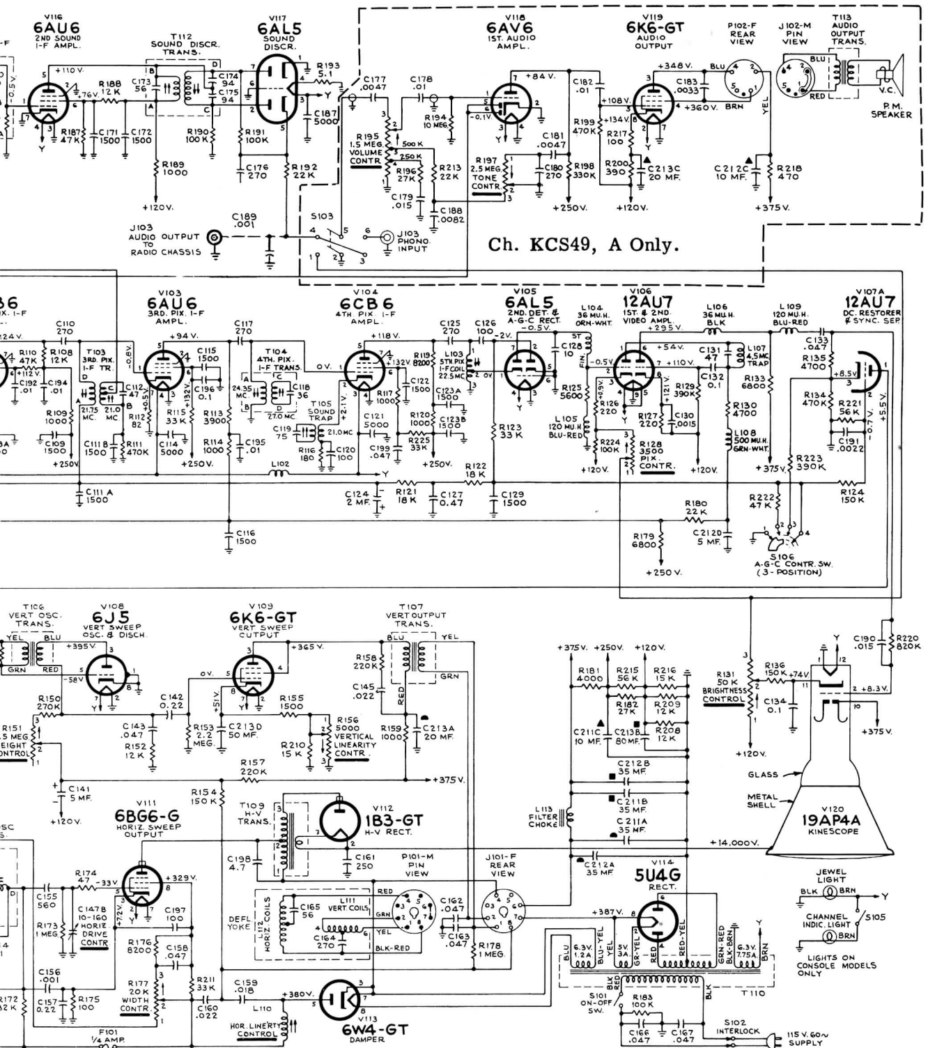
RCA VICTOR Models 9T57, 9T77, 9T79 (Ch. KCS49, A), 9T89 (Ch. KCS60)
