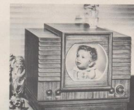
DE LUXE MODEL 1230: 12½-in. Direct-View Tube with giant 91-sq. in. Wide-View Screen. 30-tube chassis with Keyed Automatic Gain Control. Synchronized 7-in. Alnico PM Speaker. Noise-free FM sound. Power Transformer for extra safety. Attractively styled Mahogany veneer cabinet.
